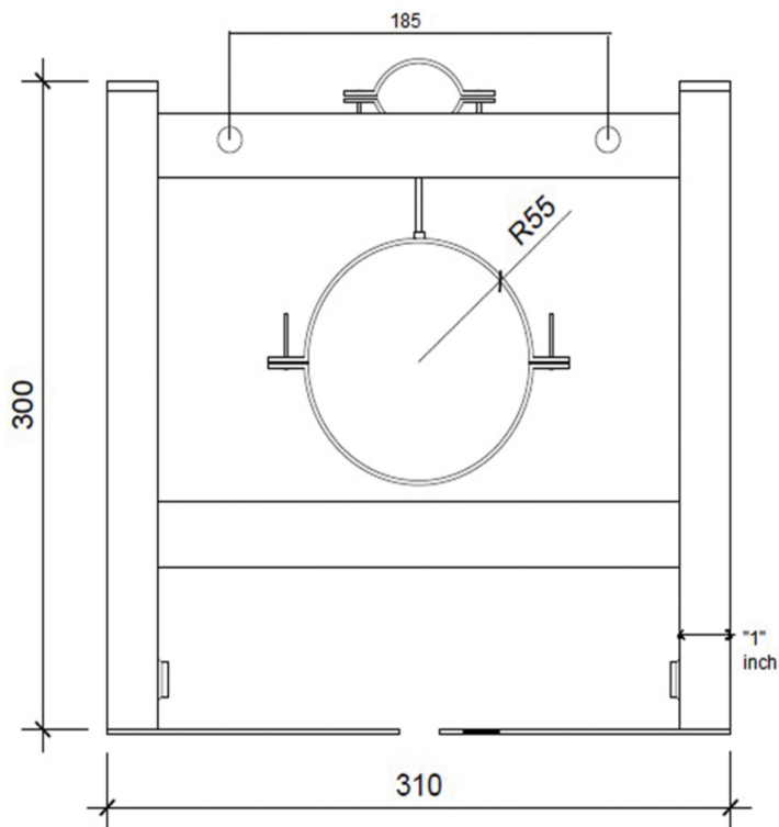
1555 WC Frame
